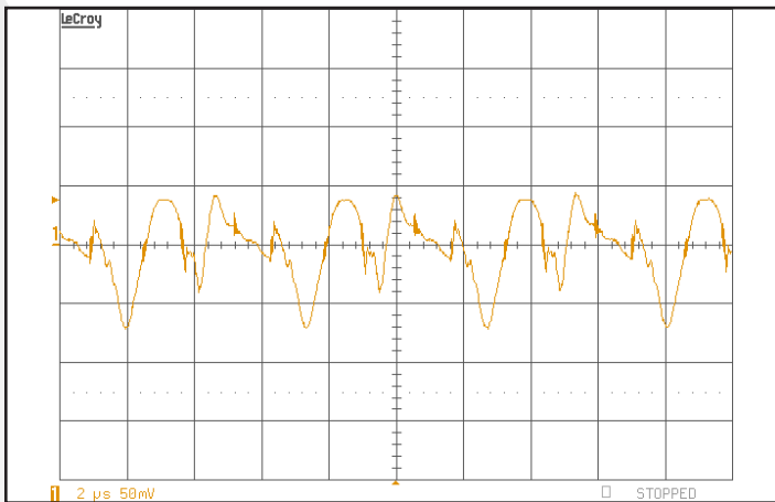
Figure 10: Output voltage ripple, Vout, at nominal input voltage and rated load current (50 mV/div). Load capacitance: 1 \mu F ceramic capacitor and 10 \mu F tantalum capacitor. Bandwidth: 20 MHz. See Figure 17.
