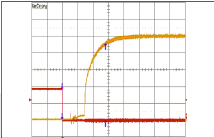
Figure 7: Typical startup waveform from enable pin. Input voltage pre-applied. Ch1: Vout (1V/div), Ch2: Enable Pin (2V/div). Horizontal Scale: 20ms/div
