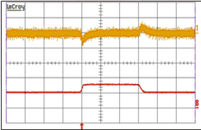
Figure 11: Output voltage response to step-change in load current (50%-75%-50% of Iout(max); di/dt = 0.1 A/\mu s ). Load cap: 1 \mu F ceramic capacitor and 10 \mu F tantalum capacitor. Ch 1: Vout (200mV/div), Ch 2: Iout (50A/div). Horizontal Scale: 1ms/div.
