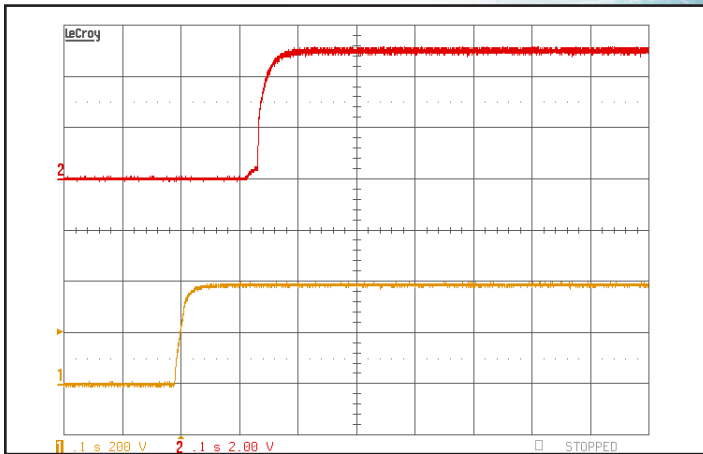
Figure 8: Turn-on transient at full resistive load and zero output capacitance initiated by Vin. ON/OFF Pin previously low. Ch 1: Vin (200V/div). Ch 2: Vout (2V/div).
