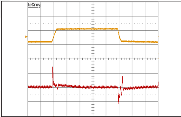
Figure 12: Output voltage response to step-change in input voltage (1V/ \mu s ). Load cap: 1 \mu F ceramic capacitor and 10 \mu F tantalum capacitor. Ch 1: Vin (200V/div), Ch 2: Vout (50mV/div). Horizontal Scale: 0.5ms/div.
